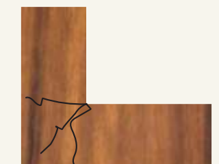
Cutting a laminate sheet at an angle of 90 degree leads to development of cracks in corner after pasting. Therefore it is advisable to avoid cutting at an angle of 90 degrees.
